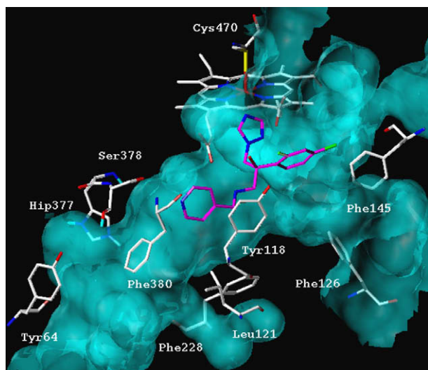
Figure 1. Docking solution of compound ( S )- 4a in the active site of CYP51- Candida albicans . His377 is the protonated form of histidine residue.
