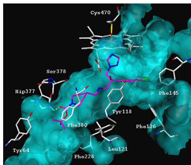
Figure 2. Docking solution of compound ( S )- 8a in the active site of CYP51- Candida albicans .
