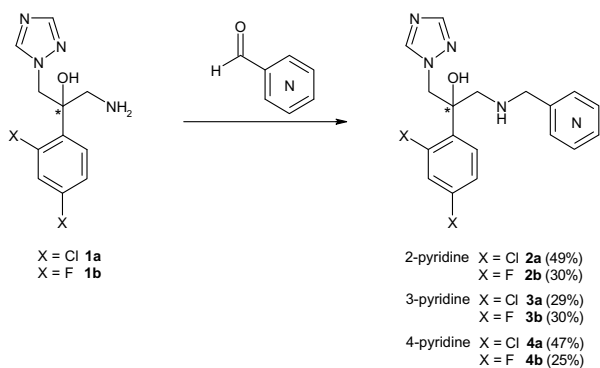
Scheme 2. Preparation of targeted compounds 2a , 2b , 3a , 3b , 4a , and 4b . Reagents and conditions: 2-pyridinecarboxaldehyde, 3-pyridinecarboxaldehyde (0.50 equiv) or 4-pyridinecarboxaldehyde (1.00 equiv), NaBH 3 CN, AcOH/MeOH 2% v/v, CH 2 Cl 2 , rt, 16 h.
