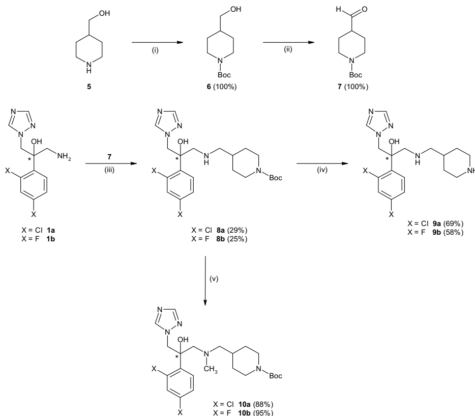
Scheme 3. Preparation of targeted compounds 8a , 8b , 9a , 9b , 10a , and 10b . Reagents and conditions: (i) Boc 2 O, CH 2 Cl 2 , rt, 1 h 30 min; (ii) oxalyl chloride, DMSO, Et 3 N, CH 2 Cl 2 , -70 °C to rt, 3 h; (iii) 7 , NaBH 3 CN, AcOH/MeOH 2% v/v, rt, 16 h; (iv) TFA, CH 2 Cl 2 , rt, 16 h; (v) HCHO, NaBH 3 CN, AcOH/MeOH 2% v/v, CH 2 Cl 2 , rt, 24 h.
