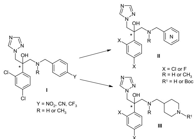
Scheme 1. General structures of synthesized compounds.
